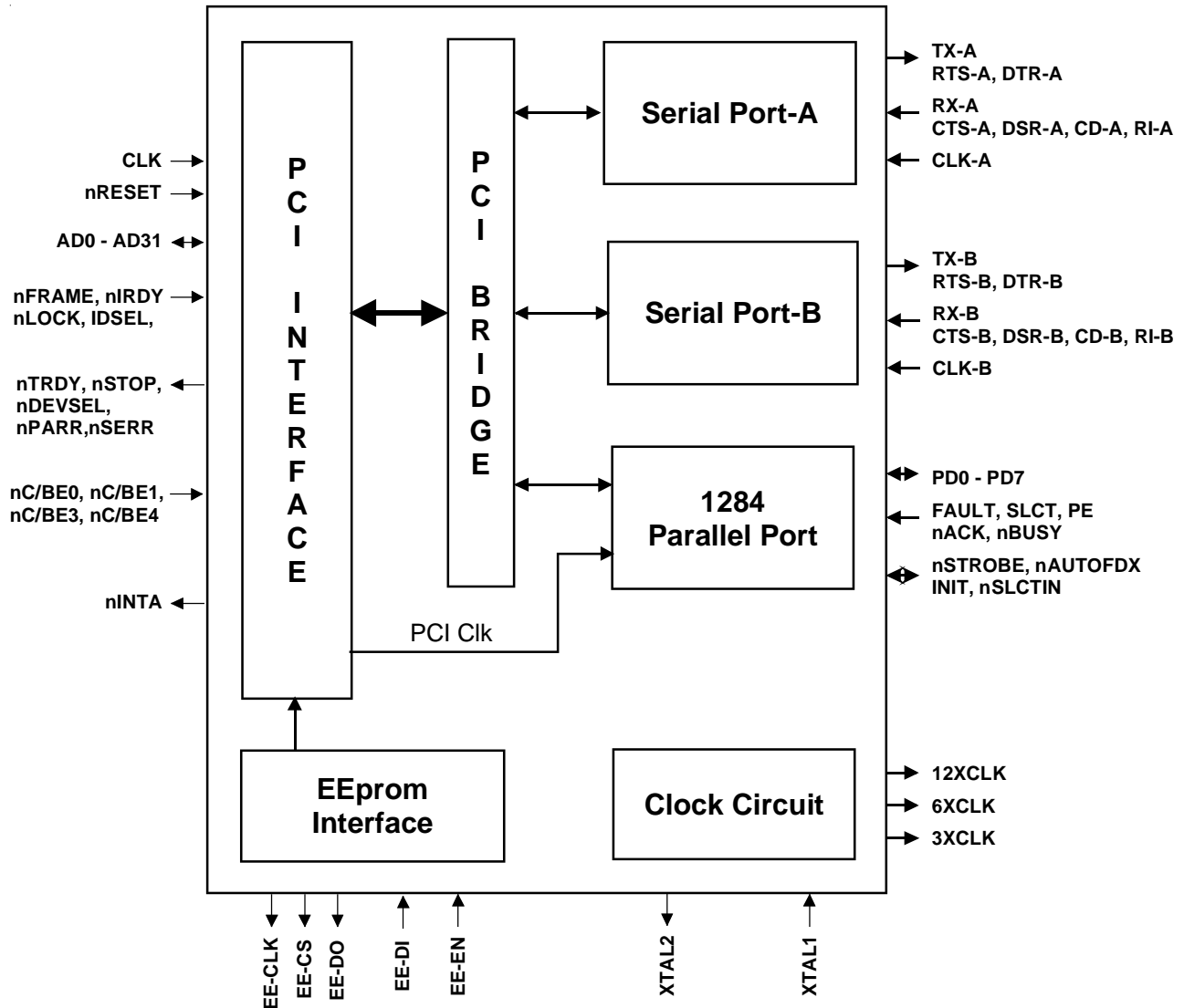
Nm9835 Block Diagram
